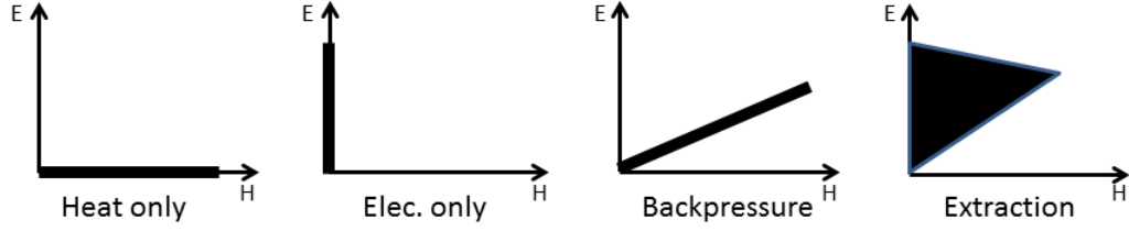
Figure 11: Operating regions for some of the energy plant types in Balmore. 'H' is heat, 'E' is electricity.
