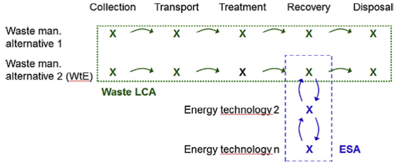
Figure 10: System boundaries of energy system analysis (ESA) and waste management life cycle assessment (LCA).
